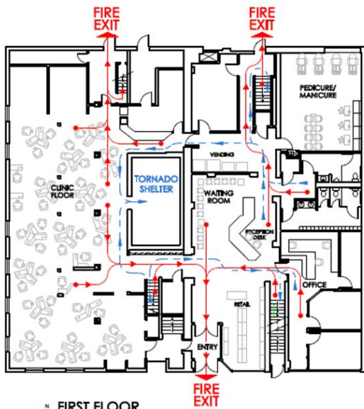
1 st FIRST FLOOR NOT TO SCALE
